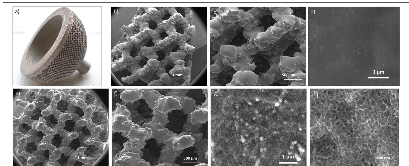
FIGURE 3 | Macroscopic appearance of the untreated cup (a) ; FESEM images of the untreated (b–d) and chemically treated (e–h) samples at different magnifications. In the treated specimens the sponge-like nanotexture resulted as homogeneously distributed onto all the cup surface.
