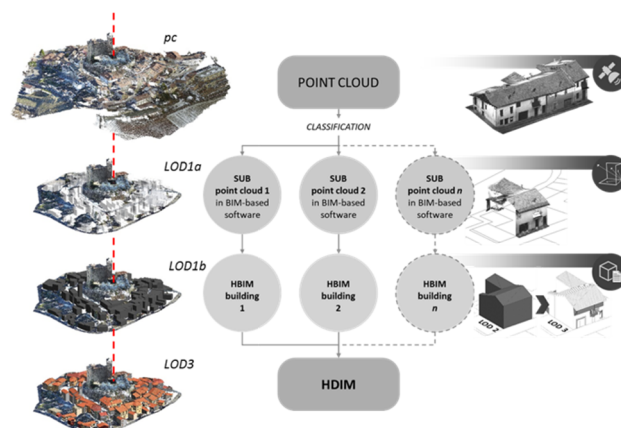
Figure 10. Schematic of the information system for planning and design management of cultural heritage
