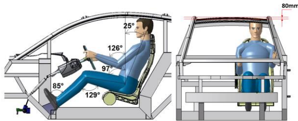
Figure 13. 3D dummy ergonomics
