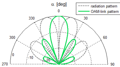
Figure 3. Solid line : OAM-link pattern (total received power in dB as a function of the rotation angle \alpha for the receiving configuration \ell_R = \ell_T = 1 ); dashed line : conventional radiation pattern for \ell_T = 1 . Both the curves are normalized to their respective maxima. It should be noted that the plotted quantities represent two distinct concepts from a physical point of view.
