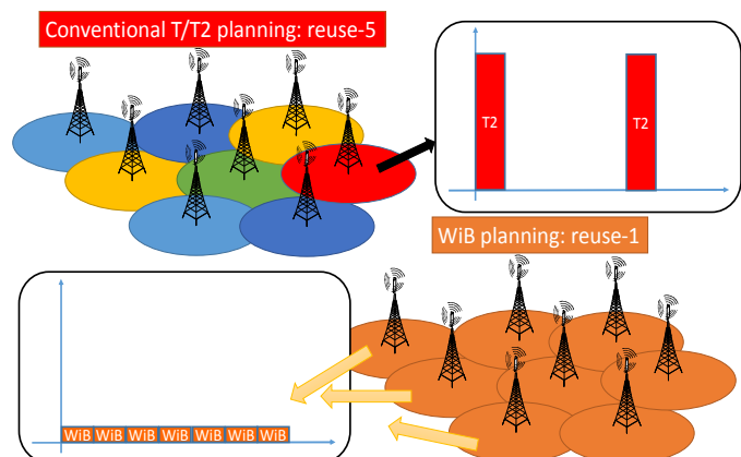
Figure 1 – Conventional vs WiB frequency planning
