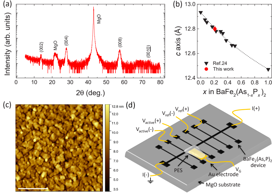
FIG. 1. (a) XRD spectrum of a \simeq 10 nm thick \text{BaFe}_2(\text{As}_{0.79}\text{P}_{0.21})_2 film. (b) Out-of-plane lattice constant c , determined from XRD, as a function of the P content x . Red circle is obtained from the spectrum in (a). Black down triangles are adapted from Ref.24. Black dashed line is a guide to the eye. (c) AFM topographic image acquired in tapping mode of the surface of the same thin film. Root mean square height is S_q \simeq 1.5 nm, much smaller than the nominal film thickness. Scale bar is 1 \mu\text{m} . (d) Sketch of a \text{BaFe}_2(\text{As,P})_2 device with the electrical connections required for double-channel four-wire resistance and gating measurements.
