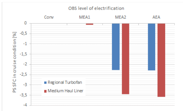
Fig. 10. Influence of OBS electrification on engine SFC.
