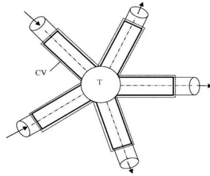
Figure 5. Schematic of the control volume of a junction node [20].
