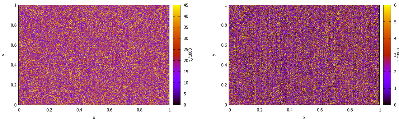
Fig. 5. Heat-maps for convergence times t_{c,\epsilon} of map (75), with \epsilon = 0.01 and 5 \cdot 10^5 samples. Each initial condition is colored depending on t_{c,\epsilon} of the corresponding trajectory. The dominant color represents the peak in Fig. 4
