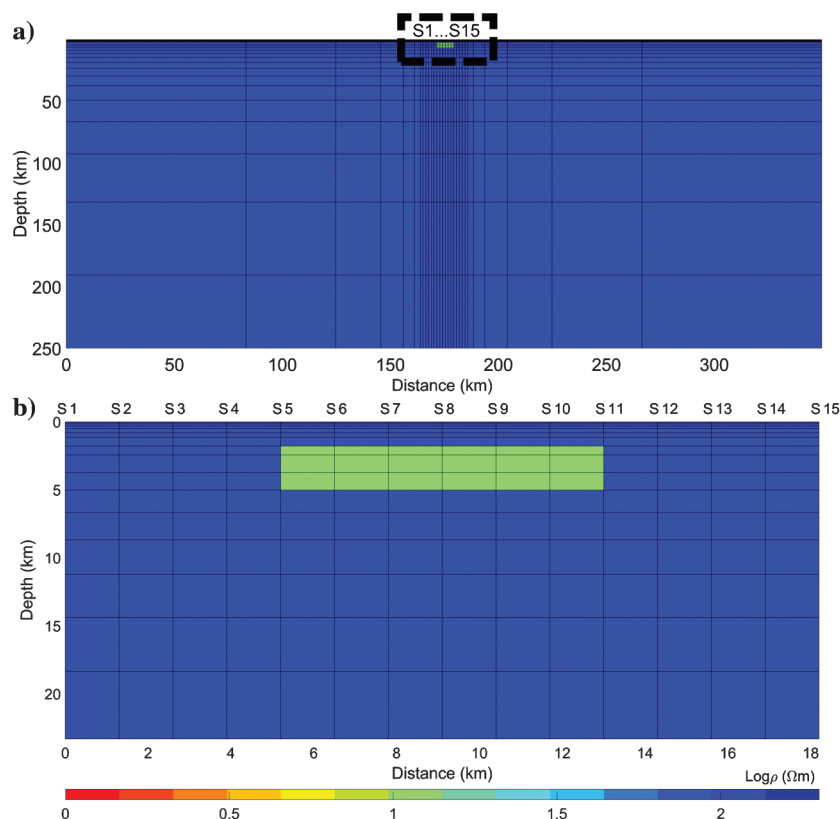
Figure 2. Synthetic model 1: (a) The 2D mesh is discretized into 33 layers and a total of 957 grid cells. The labels S1, ..., S15 indicate the location of the 15 MT stations. The dashed area is shown in (b): A 10 ohm-m conductive body is hosted in a 100 ohm-m medium.
