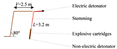
Fig. 4. Cross section of a blasthole.
