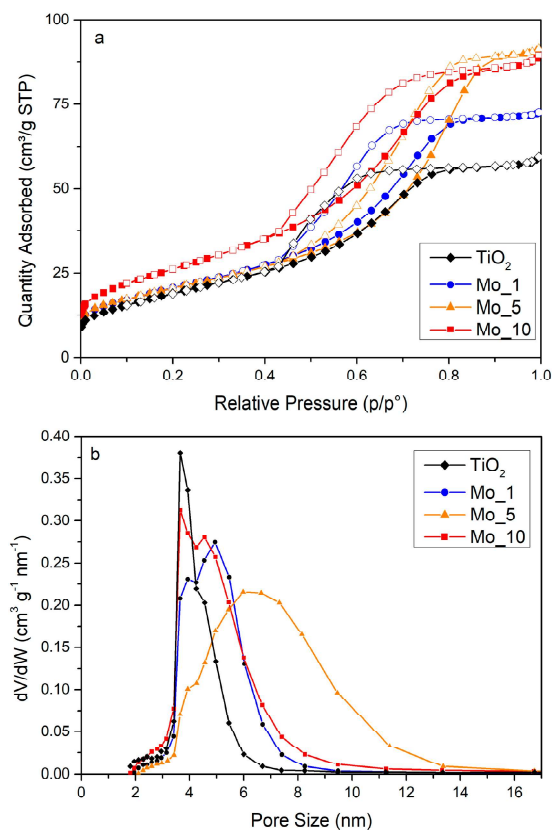
Figure 2. (a): N 2 adsorption/desorption isotherms at -196 °C (full symbols: adsorption branch; hollow symbols: desorption branch); (b): pore size distributions (PSDs) of bare and Mo-doped TiO 2 .
