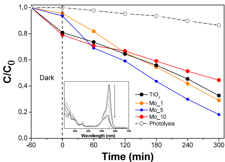
Figure 6. Relative concentration profile of RhB degradation under visible light. Inset UV–Vis absorbance spectra carried out during the photodegradation of RhB in the presence of the Mo_5 sample.
