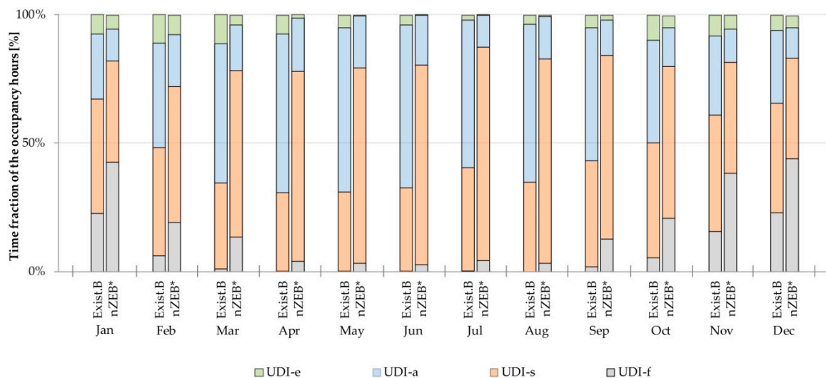
Figure 7. Comparison of the UDI levels for the occupied hours over the whole year between the building in the present configuration (Exist.B) and after the retrofiting of the building envelope (nZEB*) on a monthly basis.
