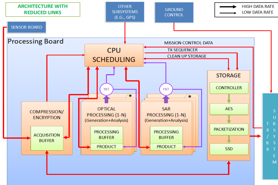
Figure 2 EO-ALERT architecture
