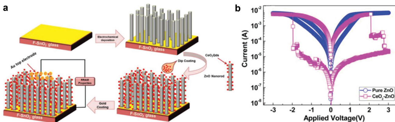
Figure 25. a) Schematic diagram for the realization of devices based on CeO_2 -ZnO nanocomposites and b) comparison of the I - V characteristic in pure ZnO NR array and CeO_2 -ZnO composites. All panels adapted with permission. [247] Copyright 2013, American Chemical Society.
