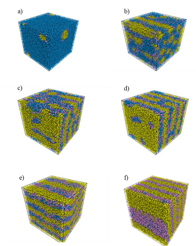
Figure 8. Snapshots of the non-equilibrium structure at long times for Pluronic L64 in water at different weight concentrations: 5% wt, 55% wt, 70% wt, 75% wt, 85% wt, 90% wt. In each snapshot, a full version comprising water (blue), PEO (pink) and PPO (yellow) beads is reported together with a lean version, where water was faded out for simplicity. The shear rate imposed on the system is equal to 0.1 DPD units.
