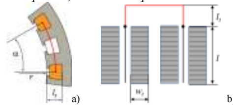
Fig 19. End-winding model used for q = 3 and q = 4/5 . a) Frontal view; b) top-view cross section.
