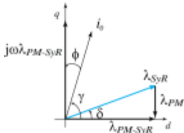
Fig 11. Vector diagram of the PM-SyR motor in natural compensation conditions.
