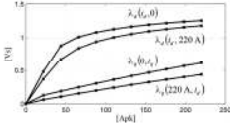
Fig 3. dq flux linkage curves of the q = 3 motor.
