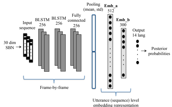
Figure 1: Example of embedding DNN architecture.
