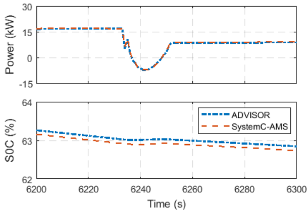
FIGURE 8. Zoom in of the evolution of computed mechanical power (top) and battery SOC over time (bottom) to highlight the impact of regenerative braking on battery SOC.
