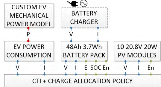
FIGURE 9. The custom EV: picture (top) and energy subsystem modeled with the proposed framework (bottom).
