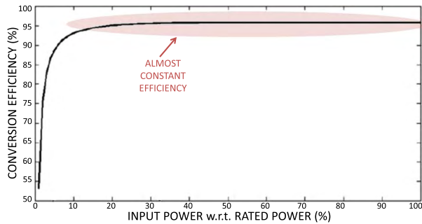
FIGURE 3. Typical efficiency curve of an inverter: efficiency tends to be constant and almost independent on input power, whenever this is at least 15% of rated power.
