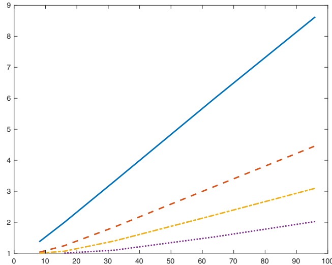
FIGURE 1. Constants C_{p,q,r} vs q = p + k for: k = 2 (solid), k = 4 (dashed), k = 6 (dashdot), k = 10 (dotted). The dependence is clearly linear rather than constant but the growth is moderate.
