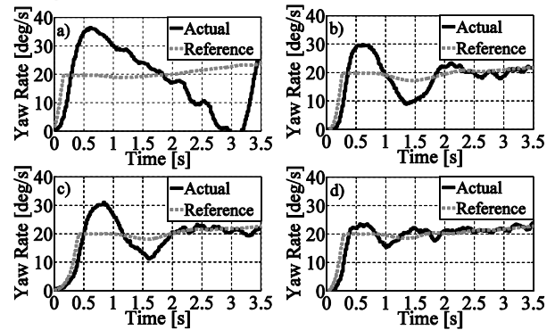
Figure 10. r(t) during a step steer for the passive (a) and active (LQR (b), LQR+FF (c) and ISMC (d)) vehicles.
