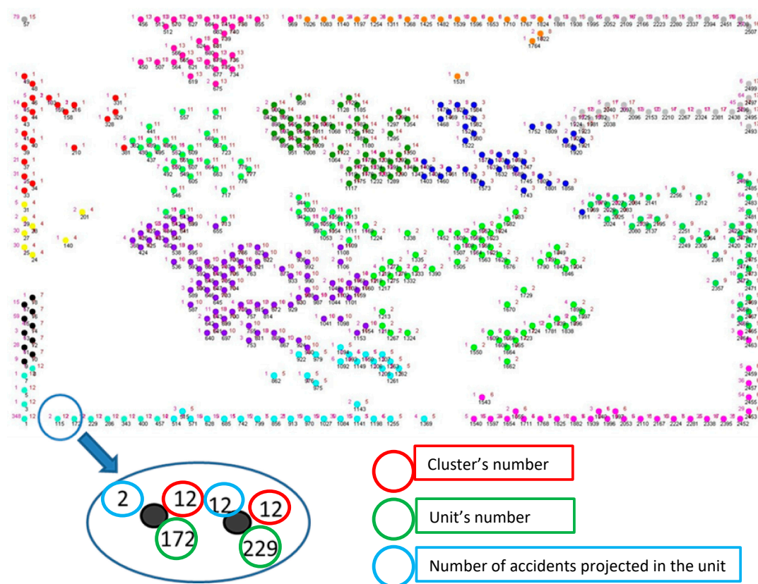
Figure 2. Partition output.
