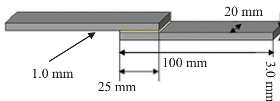
Figure 1. Single Lap Joint specimen.
