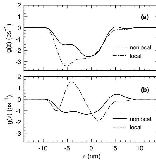
Figure 2. Time derivative of the upper-level Wigner-function profile (see Equation (49)): comparison between the nonlocal model in (44) (solid curves) and its local counterpart in (47) (dash-dotted curves) in the absence (a) and presence (b) of Pauli-blocking terms (see text).
