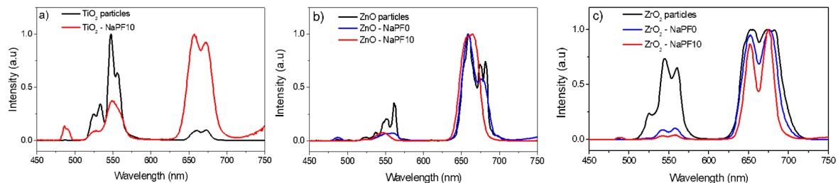
Figure 7. Normalized up-conversion emission spectra of the \text{Er}_2\text{O}_3 -doped \text{TiO}_2 (a) \text{ZnO} (b), and \text{ZrO}_2 (c) particles and of the corresponding particles-containing NaPF0 and NaPF10 glasses with 1.25 wt % of particles.
