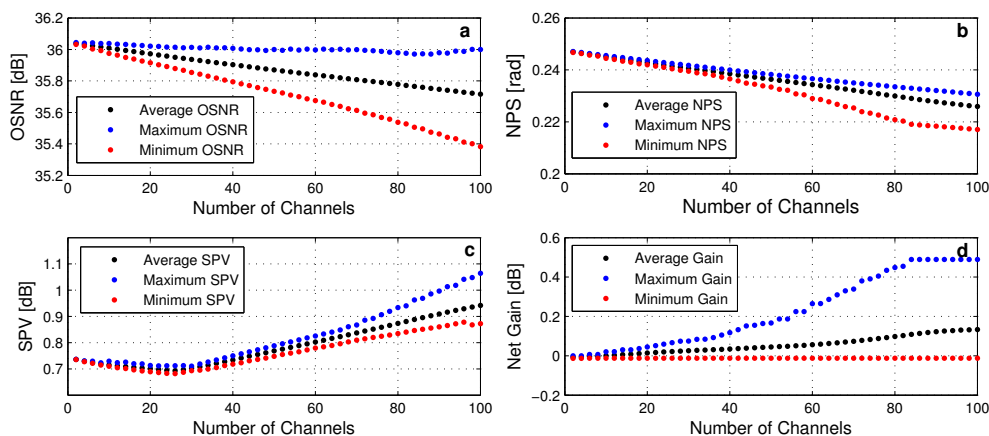
Fig. 6. The performance of the 25 GHz spaced DWDM transmission with up to 100 channels using random DFB Raman laser amplification. The received OSNR (a), NPS (b), SPV (c) and received net gain (d) are shown for the best (blue) and the worst (red) performing channels. The span length was 50 km and the launch power per channel was set to -5 dBm.
