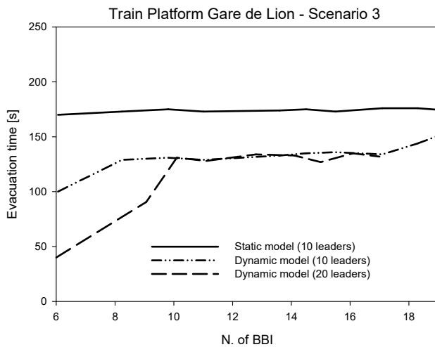
Figure 21. Comparison among the static and the dynamic leader-follower behavior models with 10 and 20 leaders for the train station.
