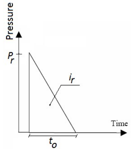
Figure 9. Idealized blast overpressure time history (adopted from TM5-1300-1990)
