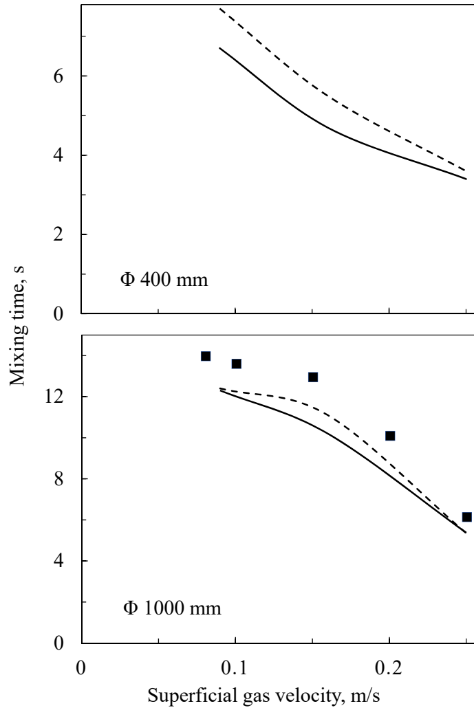
Figure 12: Mixing time as a function of the gas velocity, computed by using the RNG k - \epsilon model coupled with SIT (dashed line) and BIT + SIT (solid line). Comparison with the experimental data of Forret (2003) (■).
