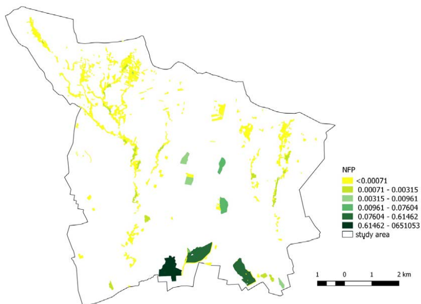
Fig.5 Spatial distribution of NFP index, showing the relative importance of single nodes for the composite multi-specie ecological network considering patch area and relations with the neighboring patches
