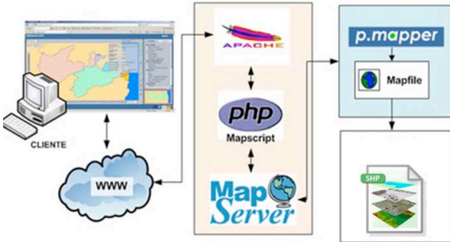
Fig. 4 The structure of the WebGIS
