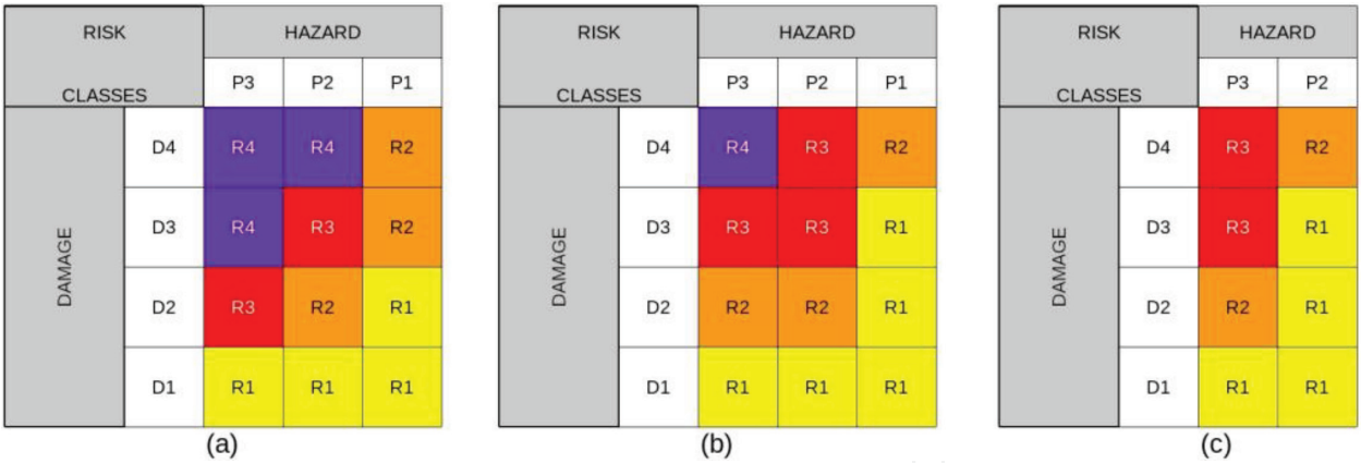
Figure 1. The matrices adopted in PGRA, by Po basin District Authority. Hazard classes P1, P2, and P3 refer to the return period indicated in EFD (P1 for T = 20–50; P2 for T = 100–200; P3 for T = 500).
