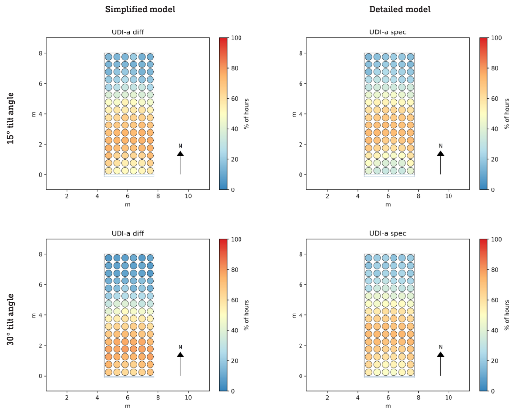
FIG. 11 UDI-autonomous (300 lux < Illuminance < 3000 lux) distribution over the sensors grid
