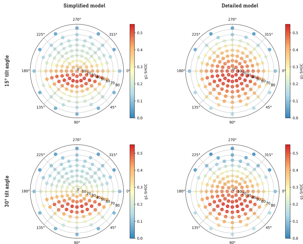
FIG. 8 Angular dependent SHGC
