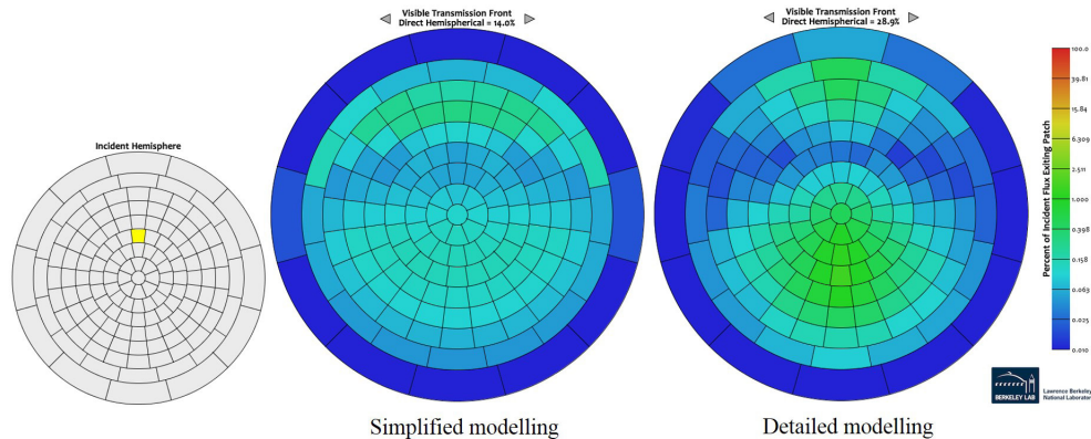
FIG. 7 BPDFs Visible Transmission Front for the fenestration system with blind tilted at 15°. The graphs show the 145 outgoing values of visible transmission for an incident ray normal to the system and at 30° of elevation (yellow patch on the first left image).
