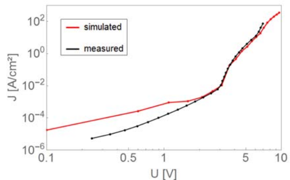
Fig. 8. Comparison between a simulated and a real I-V curve of a VDR.
