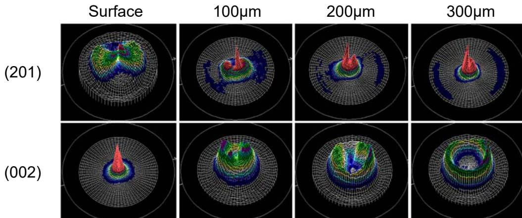
Fig. 4. Pole figures of a mirror-polished sample (ZrO 2 powder ; 900°C)
