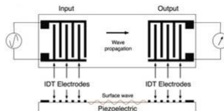
Fig. 1. Principle of SAW sensors.
