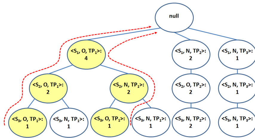
(a) Paths containing o-item \langle s_3, 0, TP_1 \rangle in the initial FP-tree
