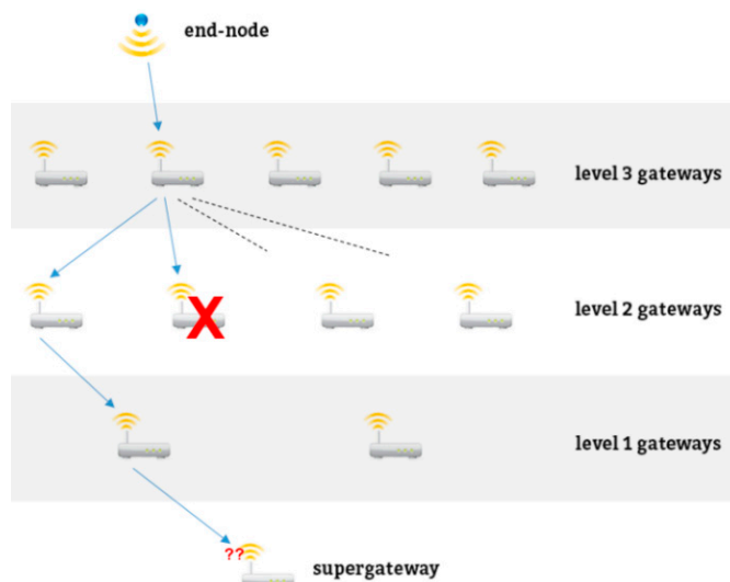
Figure 4. A hypothetical case of failure of a gateway, which results nonetheless in correct delivery of the packet and fault detection by the supergateway.
