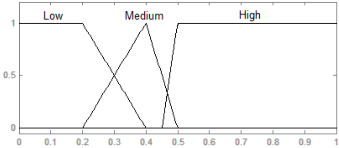
Figure 7: Membership functions of the fuzzy sets related to \bar{g} (for dataset B).
