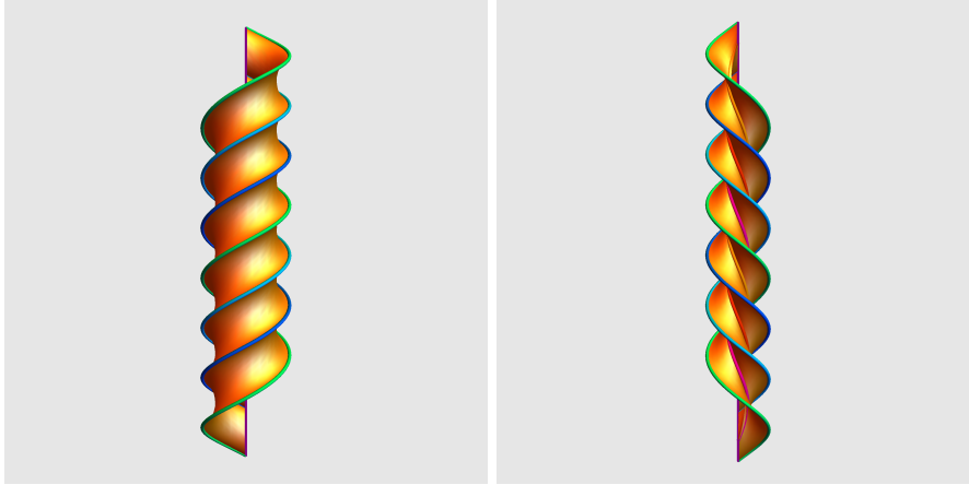
FIGURE 10. Magnetic (left) and electric (right) pseudospherical twisted columns with n = 3 and \mathfrak{d} = \phi , \phi = golden ratio.
