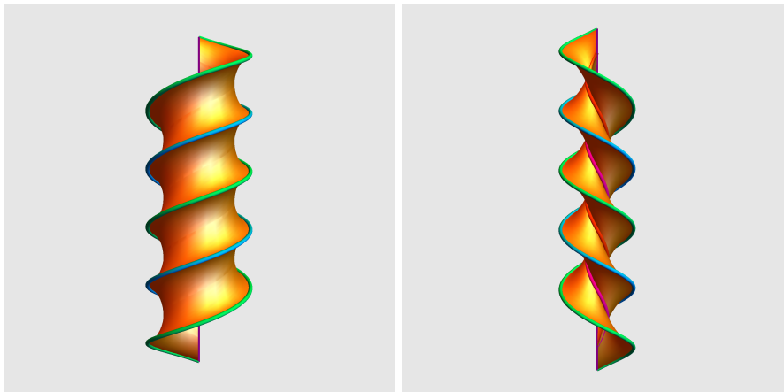
FIGURE 9. Magnetic (left) and electric (right) pseudospherical twisted columns with \mathbf{n} = 2 and \mathfrak{d} = \phi , \phi = golden ratio.
