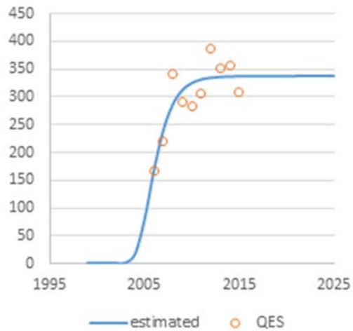
Figure 10 - Gompertz curve (Greece).
