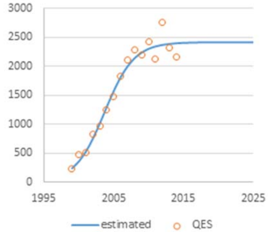
Figure 15 - Logistic curve (Spain).
