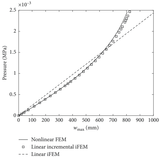
FIGURE 4: Wing-shaped plate. Load-deflection curves corresponding to the nonlinear direct FEM and linear iFEM solutions. The maximum deflection ( w_{\max} ) is located at the intersection between the tip chord and the trailing edge.
