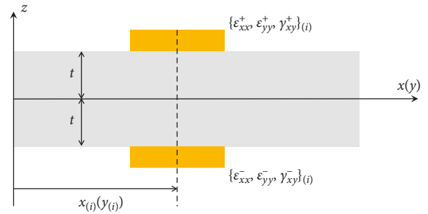
FIGURE 2: Strains measurement.
