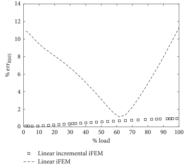
FIGURE 5: Wing-shaped plate. RMS percent error corresponding to linear iFEM and linear incremental iFEM solutions as a function of the load range.
