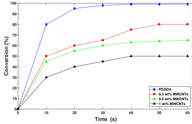
Figure 1: Conversion curves as a function of MWCNTs dispersed into PEGDA.
