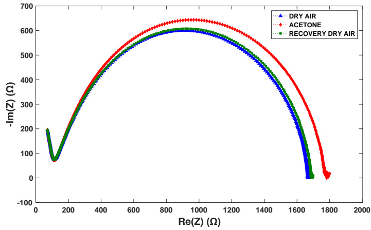
Figure 3: Static analysis of MWCNTs-based sensor with relative Nyquist plots.
