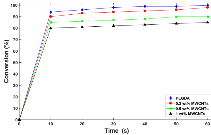
Figure 2: Conversion curves as a function of MWCNTs dispersed into PEGDA.
