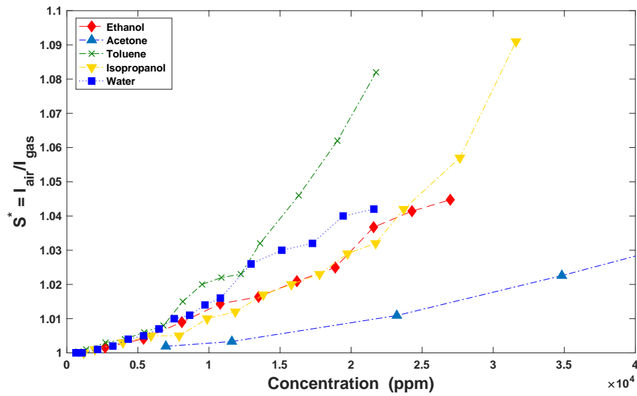
Figure 5: Sensitivity as a function of gas content for the different tested gas analytes.
