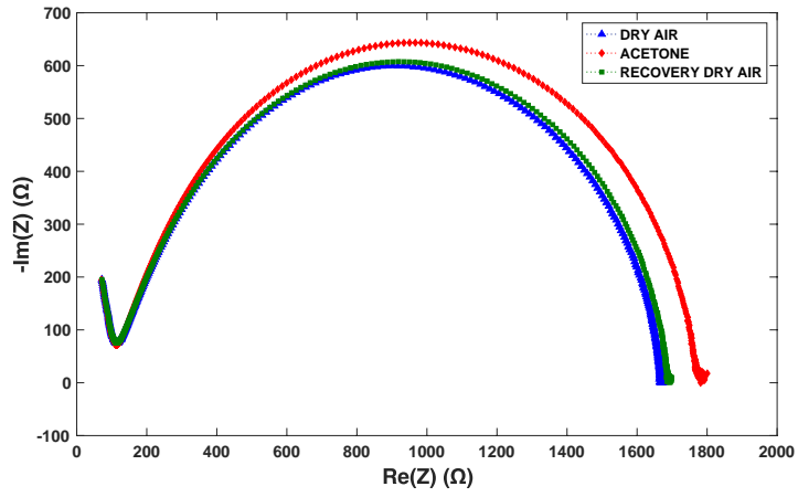
Figure 3: Static analysis of MWCNTs-based sensor with relative Nyquist plots.
