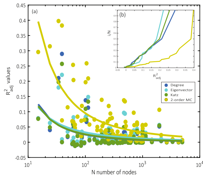
Figure 3. (a) Values of the coefficient of determination R_a^2 , in semi-log scale obtained through the centrality-based estimators degree, eigenvector, Katz and multi-component (MC). Each dot refers to a network in the Sparse Matrix database 43 . Power-law curves are fitted to the data to facilitate visual comparison. (b) Cumulative frequency curves for the R_a^2 obtained by the four estimators.
