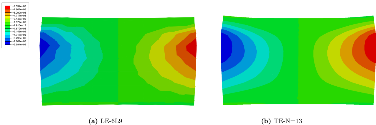
Figure 14: Cross-section displacement field u_x (m) at mid-span of the beam at t = 6.5 ms for the composite sandwich beam problem
