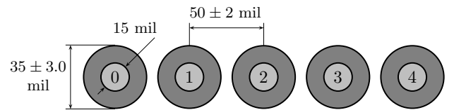
Figure 2: Cross-section of the ribbon cable for the first application test case. The deviations indicated are intended as standard deviations of a Gaussian distribution.
