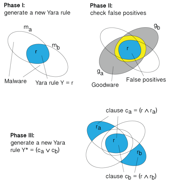
FIGURE 3. Schema of the process of generation of a YARA rule. In the first phase a signature Y = r is defined for malware m_a and m_b . In the second phase Y is checked against a dataset of goodware ( g_a and g_b ). Finally, in the third phase, a new signatures Y^* = (r \wedge r_a) \vee (r \wedge r_b) is created to avoid false positive detection of g_a and g_b .
