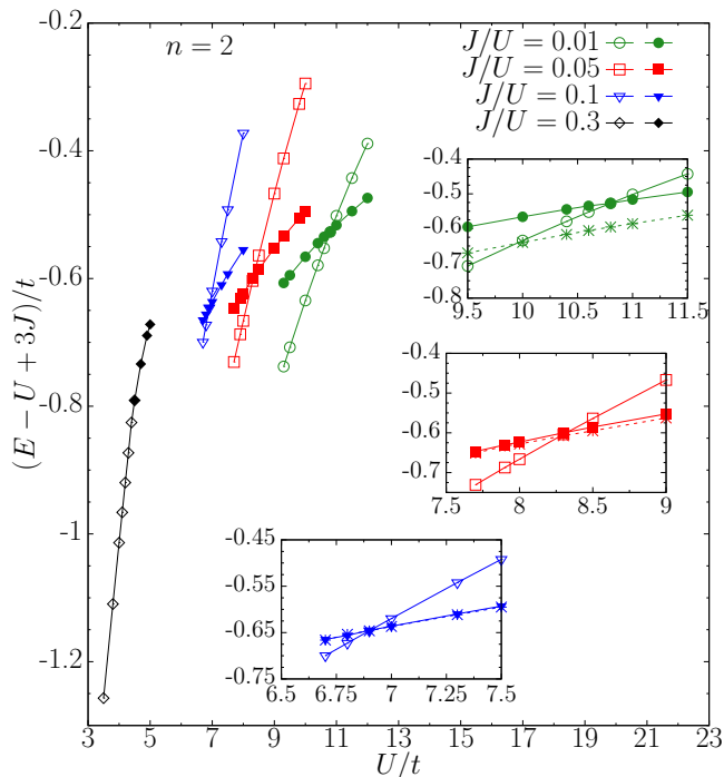
FIG. 1. Main panel: Energies (per site) of the metallic (empty symbols) and insulating (full symbols) states as a function of U/t for n = 2 and different values of the Hund coupling J ; for clarity a constant shift of U - 3J , which is the ground-state energy (per site) in the U/t \rightarrow \infty limit, has been considered. For J/U = 0.01 , 0.05 , and 0.1 the transition is first order, while for J/U = 0.3 it is continuous. No magnetic or orbital orders are considered within the variational wave functions. Insets: zooms around the metal-insulator transitions. The stars denote the energies of the insulating state when \Delta_d is allowed in the variational state.
