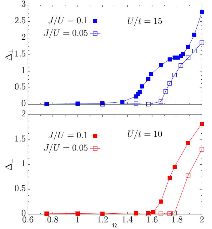
FIG. 8. Triplet pairing \Delta_{\perp} in the auxiliary Hamiltonian of Eq. (6) when no magnetic or orbital order is considered. Results are reported for U/t = 15 (upper panel) and U/t = 10 (lower panel) for two values of the Hund coupling J/U = 0.05 (empty squares) and J/U = 0.1 (full squares).
