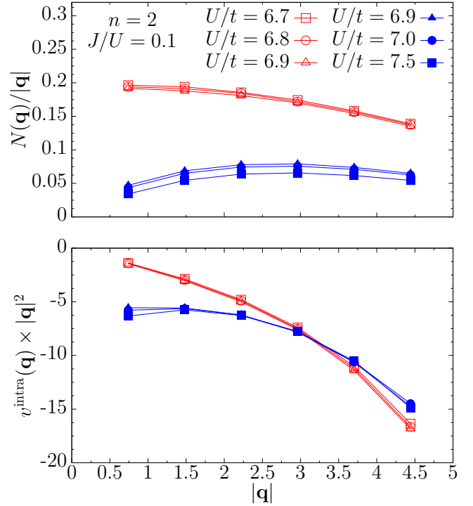
FIG. 2. Results for n = 2 and J/U = 0.1 . Upper panel: Density-density structure factor N(\mathbf{q}) of Eq. (10) (divided by |\mathbf{q}| ) for various values of U/t . Lower panel: The Fourier transform of the intraorbital Jastrow factor v^{\text{intra}}(\mathbf{q}) (multiplied by |\mathbf{q}|^2 ) for the same set of parameters as in the upper panel. The results for metallic (insulating) wave functions are denoted by empty (full) symbols. No magnetic or orbital orders are considered within the variational wave functions.
