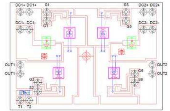
Fig. 3. Layout of the power module. In green the two internal capacitors. In blue the embedded NTC resistor (labelled "Th") measuring the DBC temperature (courtesy of Vishay Semiconductor Italiana).
