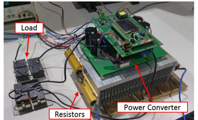
Fig. 5. Picture of the prototypal experimental setup.
