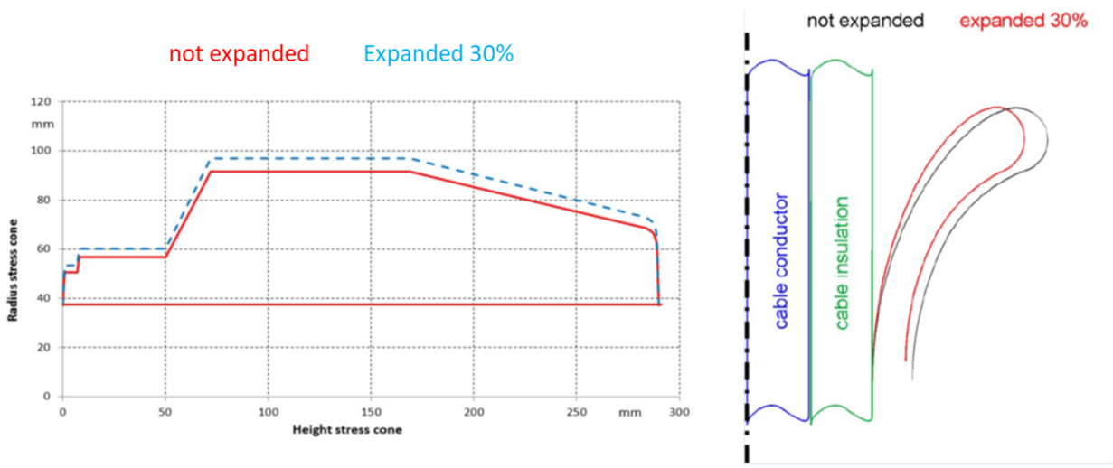
Fig. 15 Illustration of the deformation of a stress cone and a deflector with and without expansion [32]
